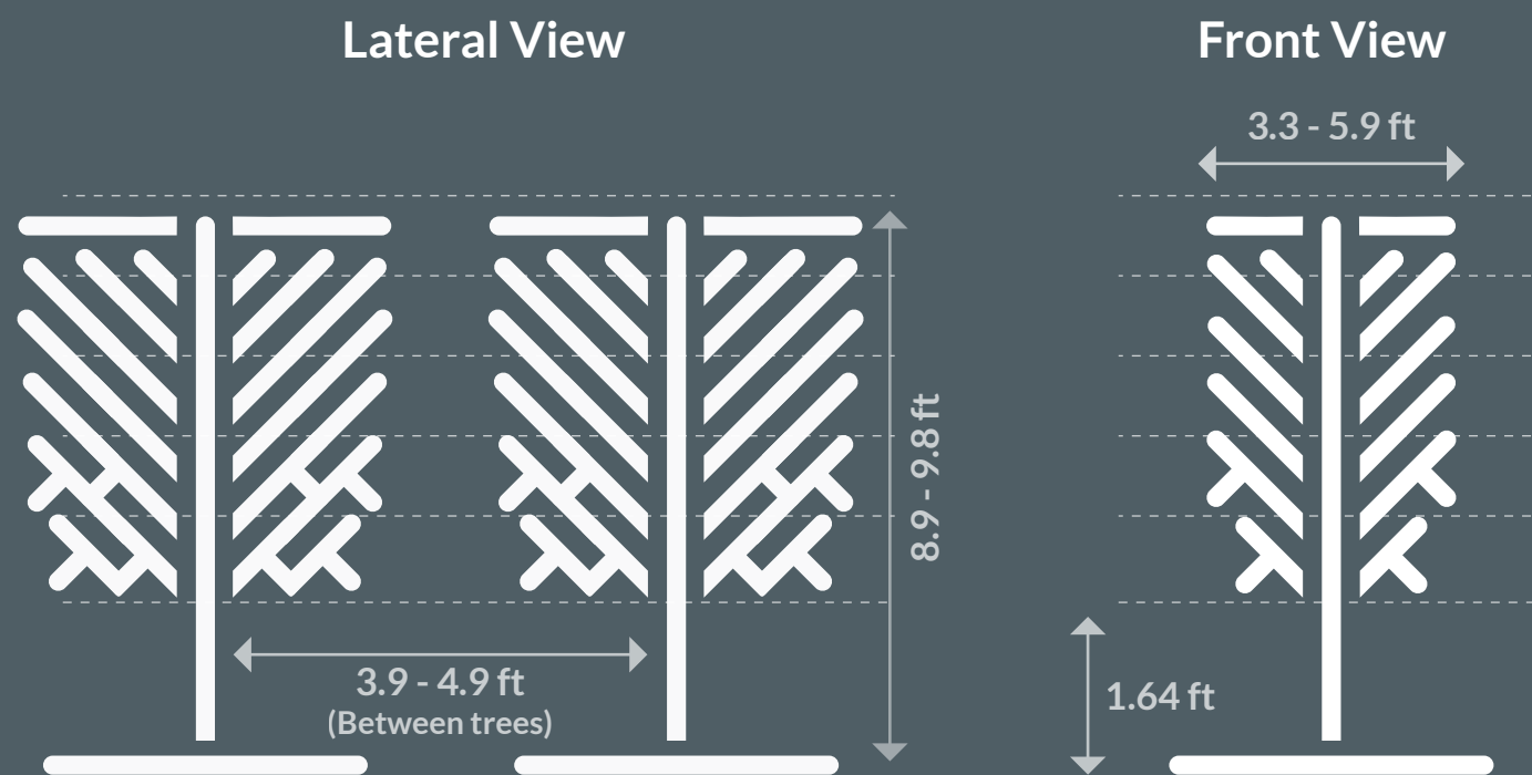
Hedge citrus dimensions with the proposed planting distances, tree width and tree height
